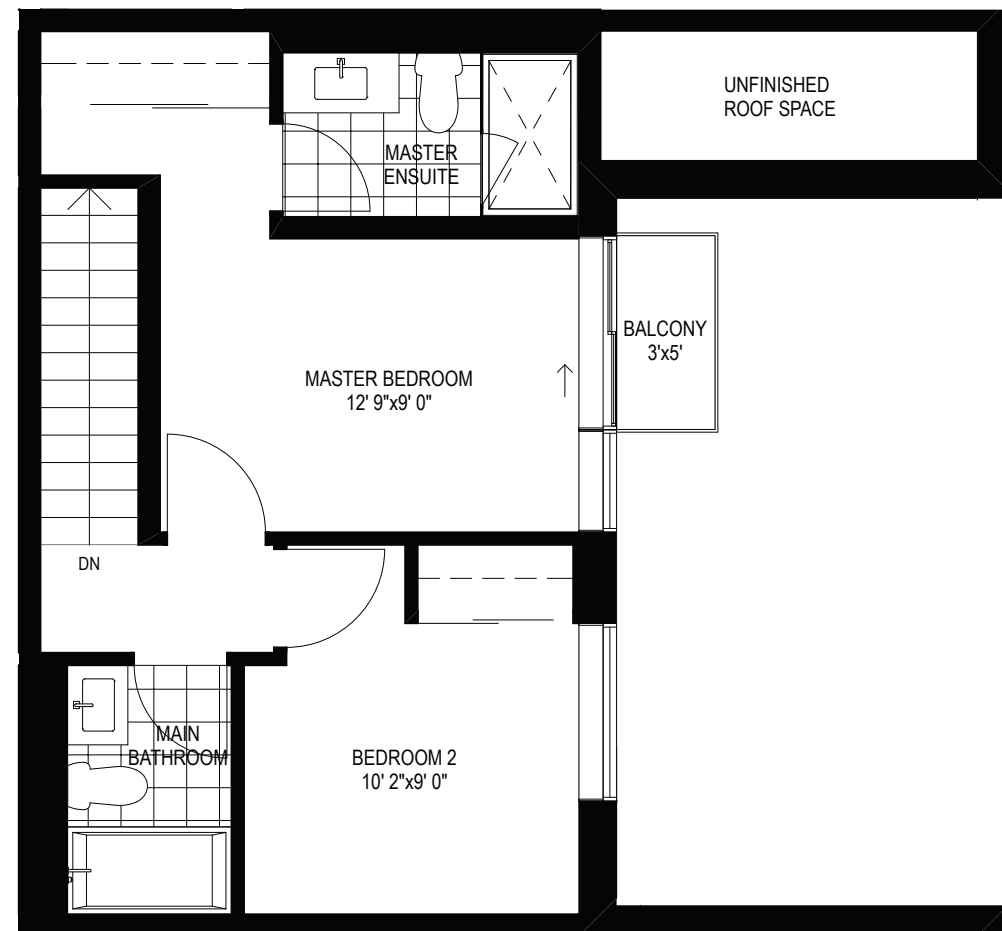
LEVEL 3
