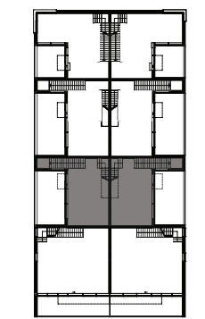
SECOND LEVEL
