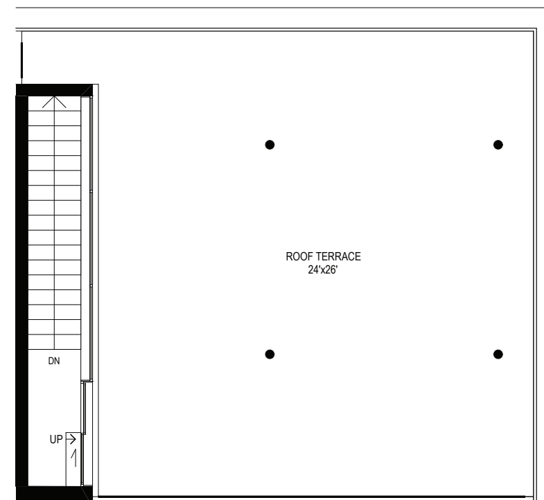
ROOF LEVEL
