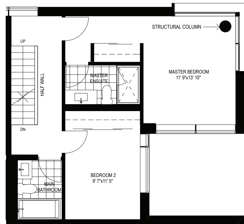
LEVEL 3
